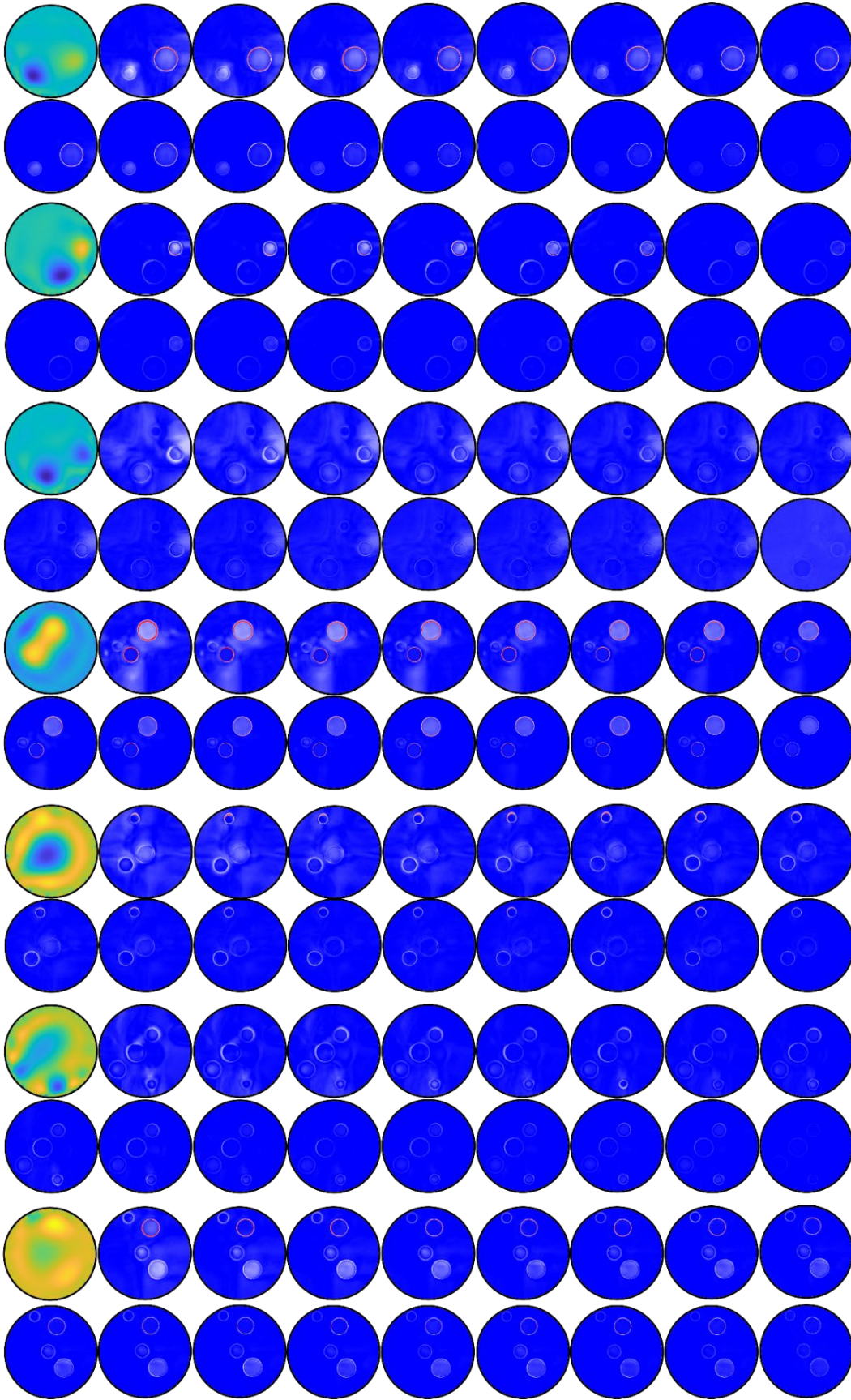
Fig. S4 The absolute error maps of reconstruction results under the multi-phase inclusions distributions of simulated test datasets , which shows the absolute error maps between the reconstruction and the ground truth. Here, the first image shows the ground truth distribution, and the last image shows the results of our SpW-Net, respectively. The other images are results of different comparisons including FISTA-Net, VA-Net, EED, DHU-Net, SWISTA-Net, PDCISTA-Net, SwinIR, Restormer, UFormer, IDT, DnSwin, DRSFormer, MWDCNN, WSDFormer, EWT, DECS-Net.
