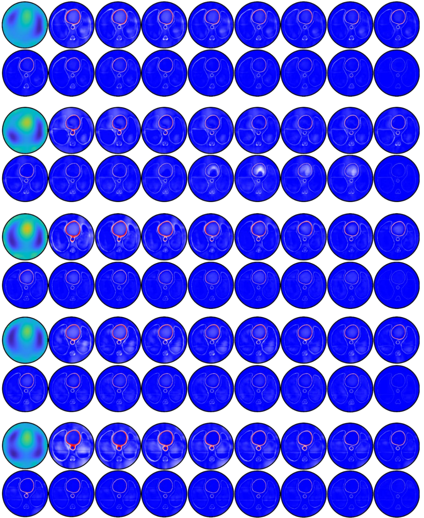
Fig. S6 The absolute error maps of reconstruction results under the lung-shaped phantoms of simulated test datasets which shows the absolute error maps between the reconstruction and the ground truth. Here, the first image shows the ground truth distribution, and the last image shows the results of our SpW-Net, respectively. The other images are results of different comparisons including FISTA-Net, VA-Net, EED, DHU-Net, SWISTA-Net, PDCISTA-Net, SwinIR, Restormer, UFormer, IDT, DnSwin, DRSFormer, MWDCNN, WSDFormer, EWT, DECS-Net.
