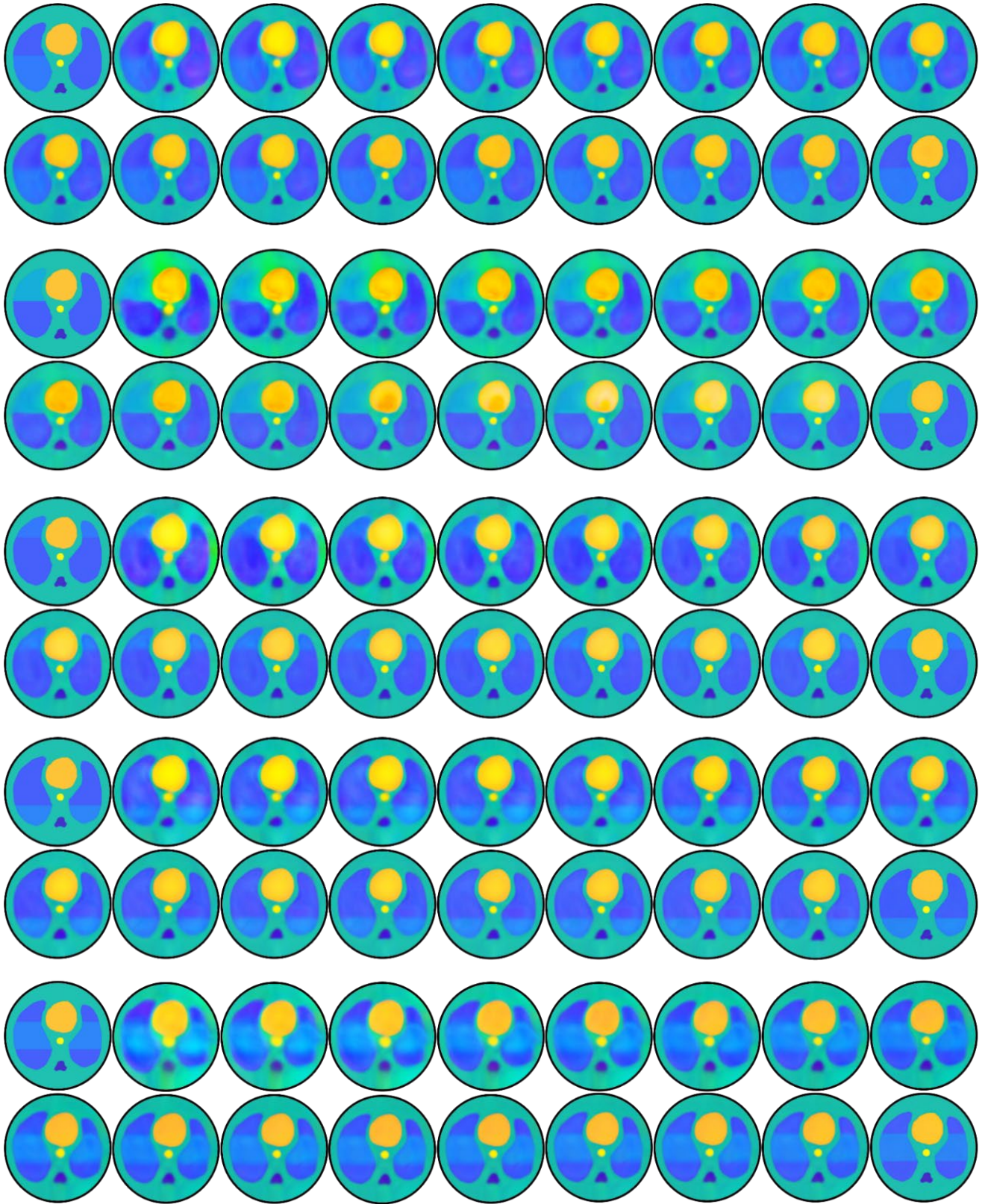
Fig. S5 The visualizations of reconstruction results under the lung-shaped phantoms of simulated test datasets . In each group, the first and second row indicate the reconstructed images. Here, the first image shows the ground truth distribution, and the last image shows the results of our SpW-Net, respectively. The other images are results of different comparisons including FISTA-Net, VA-Net, EED, DHU-Net, SWISTA-Net, PDCISTA-Net, SwinIR, Restormer, UFormer, IDT, DnSwin, DRSFormer, MWDCNN, WSDFormer, EWT, DECS-Net.
